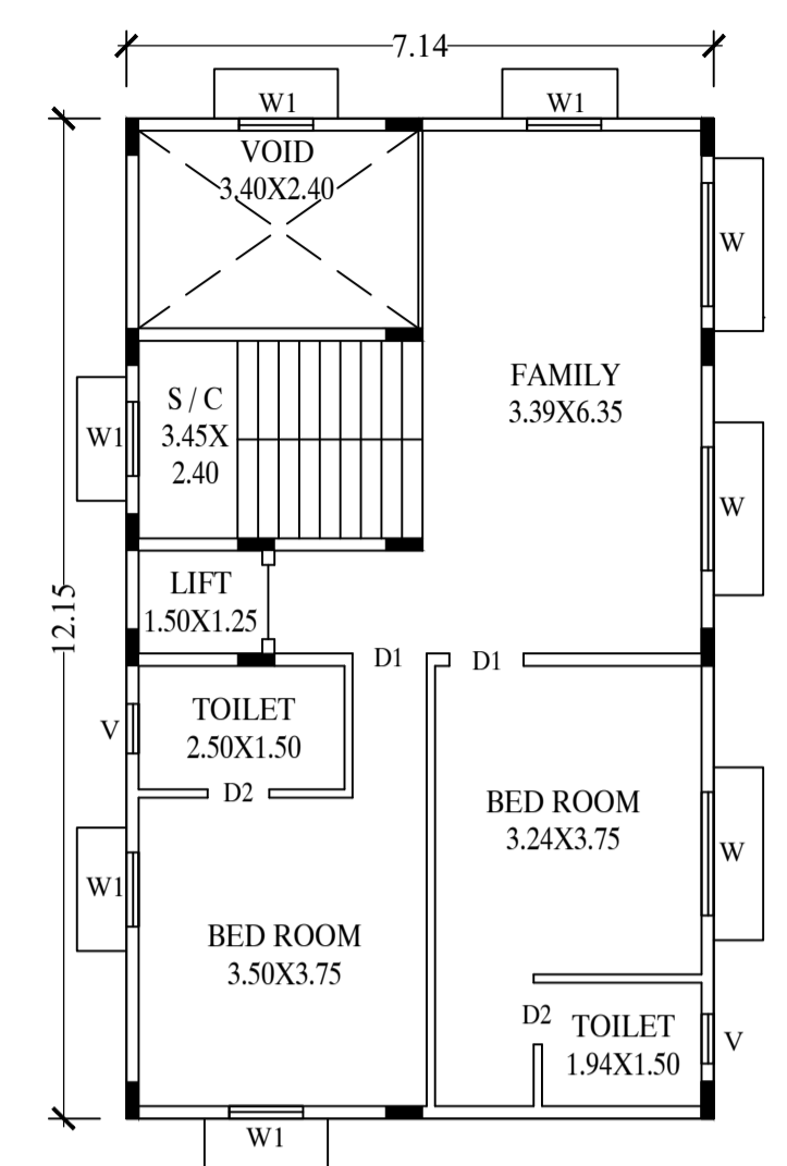
PROPOSED TYPICAL FIRST & SECOND FLOOR PLAN
